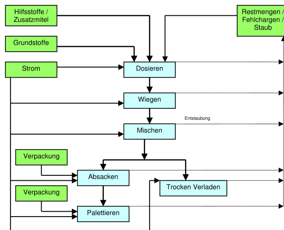
Graphic 1: Manufacturing process (green: input; blue: unit process)
