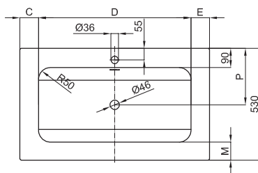
BetteOne 900 x 530 mm
