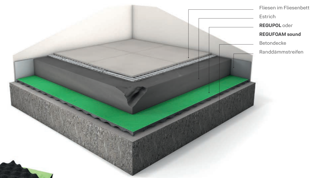
REGUPOL sound
