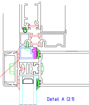
Adapterprofil Typ A 17/20 Fixing adaptor type A: 17/20
