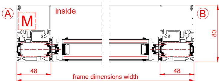
Frame type 1
