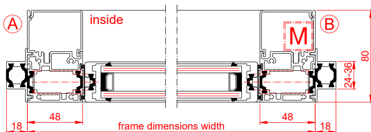
Frame type 2
