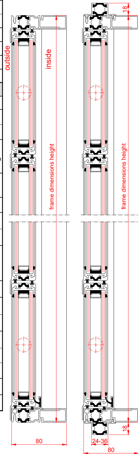
Frame type 1
