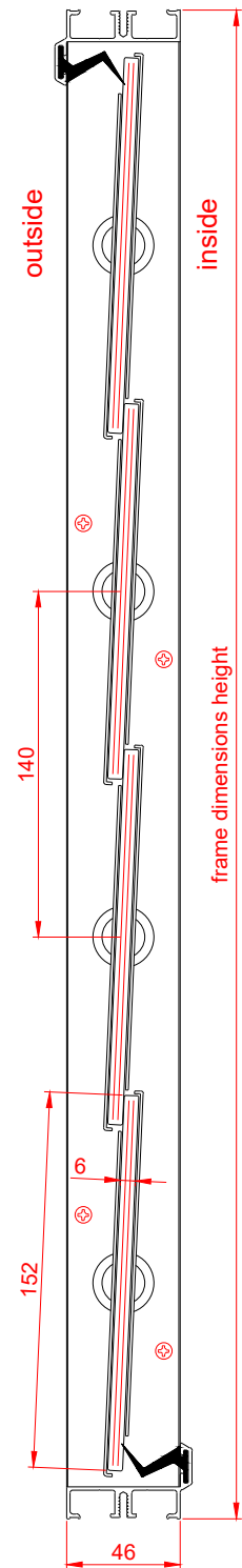
Detail glazingprofile
