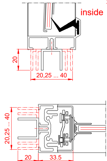
Detail glazingprofile
