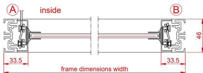
Frame type 1
