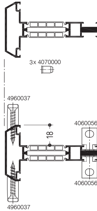
Sprosse / Sprosse Glazing bar / glazing bar
