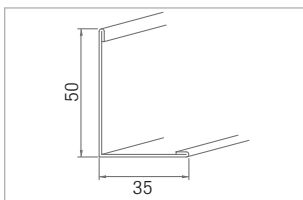
Nr. 51/1 1,0 mm dick
