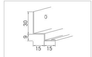
Nr. 50/22 1,0 mm dick, gelocht
