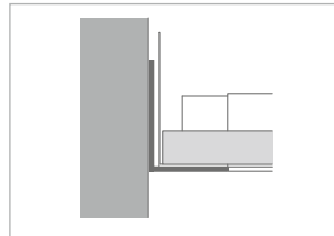
Nr. 51/1 Bandrasterdecken System S 18p/k
