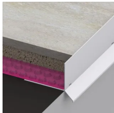
alferbal Drainage-Profil
